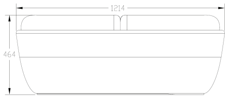
DOUBLE SEATER BENCH
