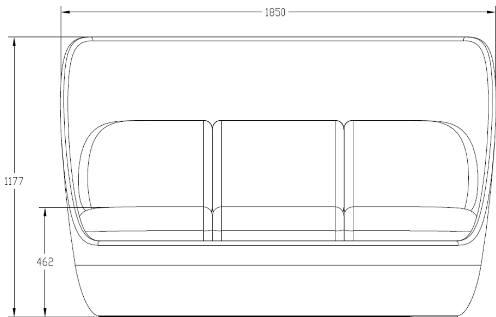
HIGH BACK THREE SEATER
