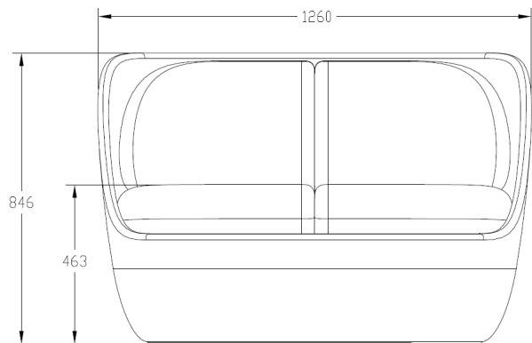
LOWER BACK TWO SEATER
