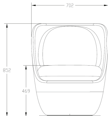
LOWER BACK SINGLE SEATER
