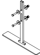
Stabilizer Support Foot (mid-run) 48.0866.XX
