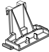
Raceway Hinge Clip 48.0103
