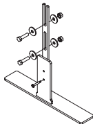
Stabilizer Support Foot (end-of-run) 48.0856.XX
