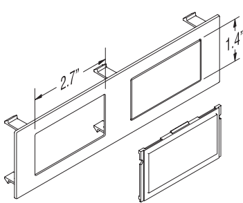
Unite Power & Data Bezel with Removable Filler Plates
