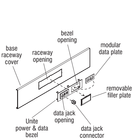
Unite Data/Communication Components
