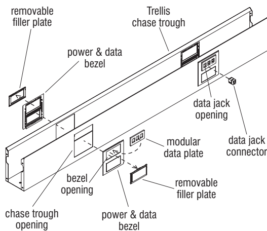
WireWorks & Trellis Data/Communication Components
