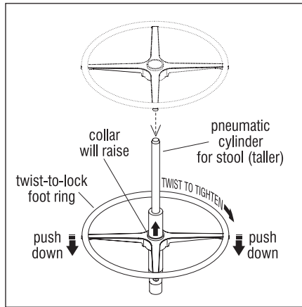
Detail A - Stool Foot Ring
