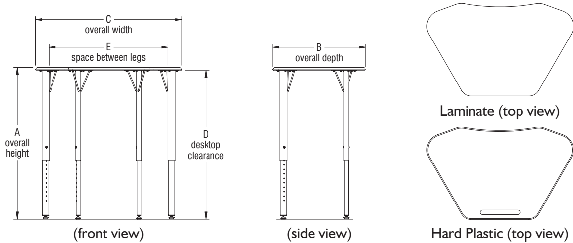
Intellect Wave - Adjustable-Height Tripod Desk - (model IWD3LCA shown)
